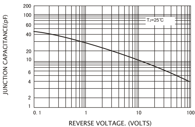
FIG.5-TYPICAL JUNCTION CAPACITANCE
